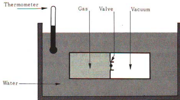
Experimental setup for studying the free expansion of a gas.
