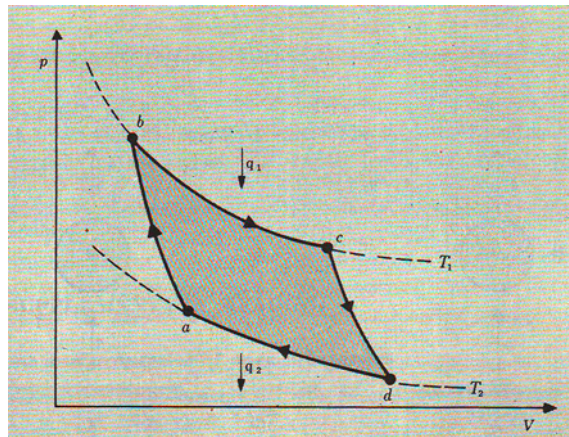
Fig. 5·11·5 The four steps of a Carnot cycle in which a gas is used as the working substance. The external parameter x is the volume V of the gas.
