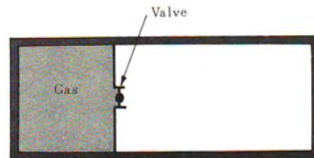
Free expansion of a gas.
